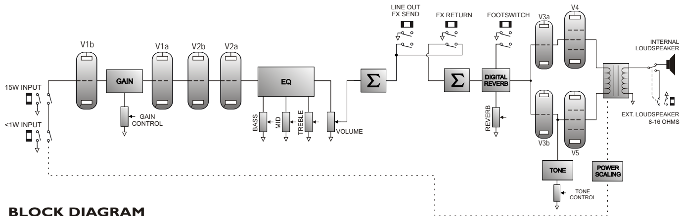
BLOCK DIAGRAM
