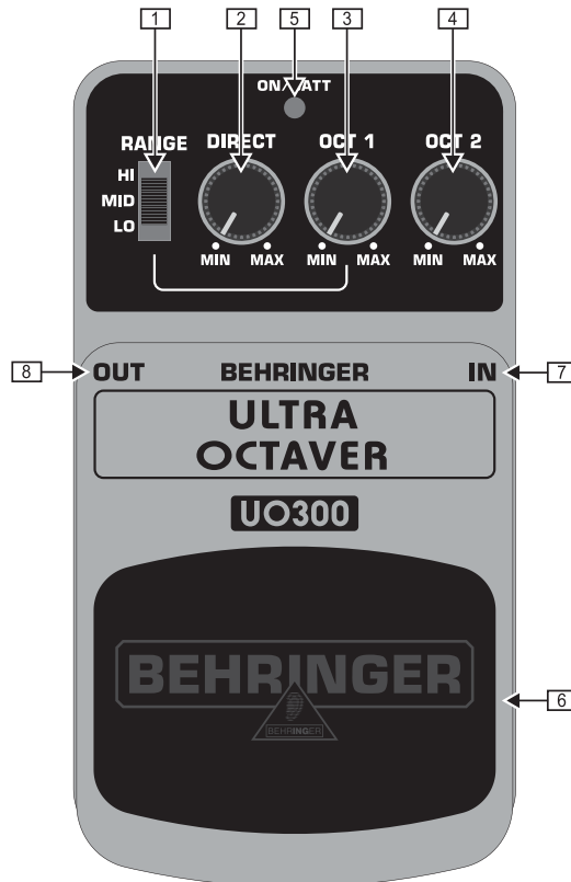
Top view
