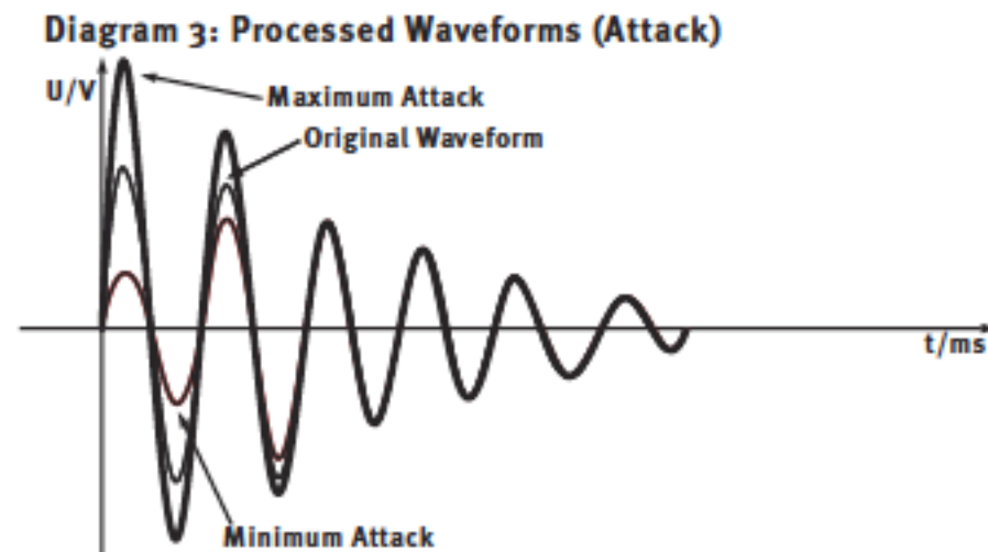
Figure 112. SPL Transient Designer Processed Attack
