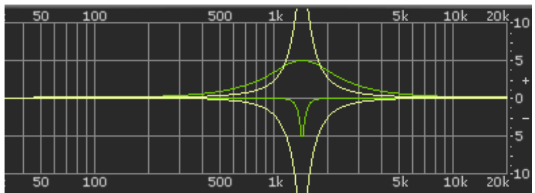
Figure 62. Parametric Type II response
