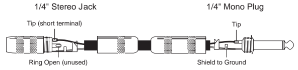
STEREO TO MONO ADAPTER
