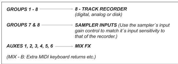
Fig. 14.1: Send routing
