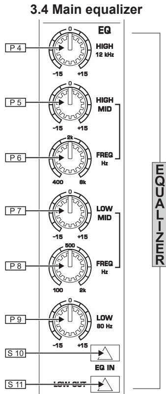
Fig. 3.3: Main equalizer
