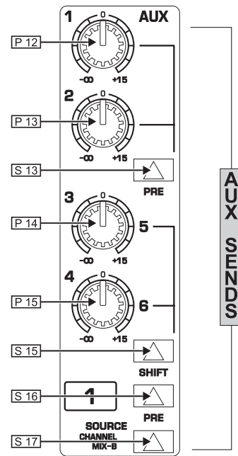
Fig. 3.4: Aux sends
