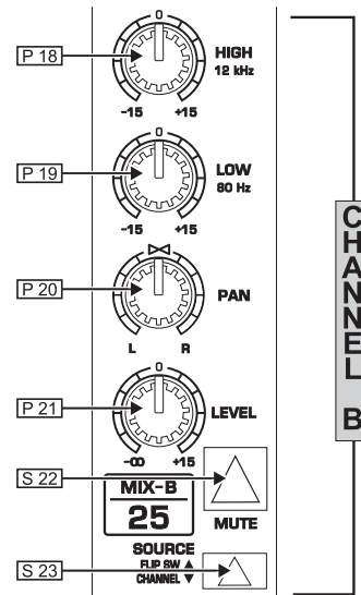
Fig. 3.6: B-channel
