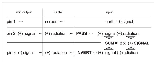
Fig. 12.1: A balanced microphone line
