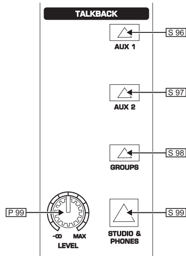
Fig. 6.7: Talkback
