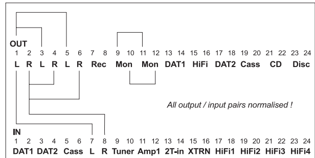
Fig. 8.4: Wiring for bay 8 (for advanced wiring scheme refer to section 11)
