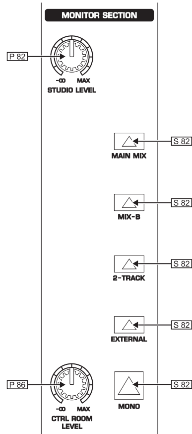
Fig. 6.4: Monitoring
