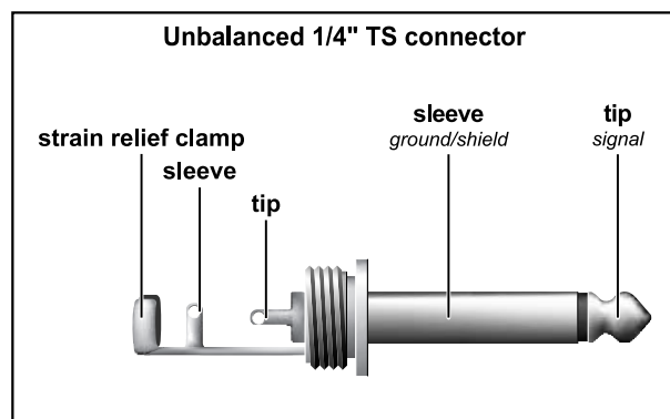
Fig. 4.1: 1/4" mono connector (TS) for the INSTR. INPUT
