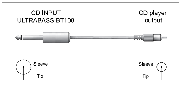
Fig. 4.4: Mono adapter cable
